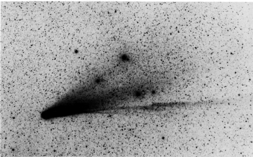
Figure 11. JOCR photographs of comet West on April 1, 1976, showing tailward motion of a kink. See text for discussion.
